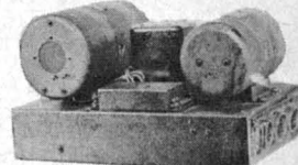
TCS POWER SUPPLY COLLINS 21881
