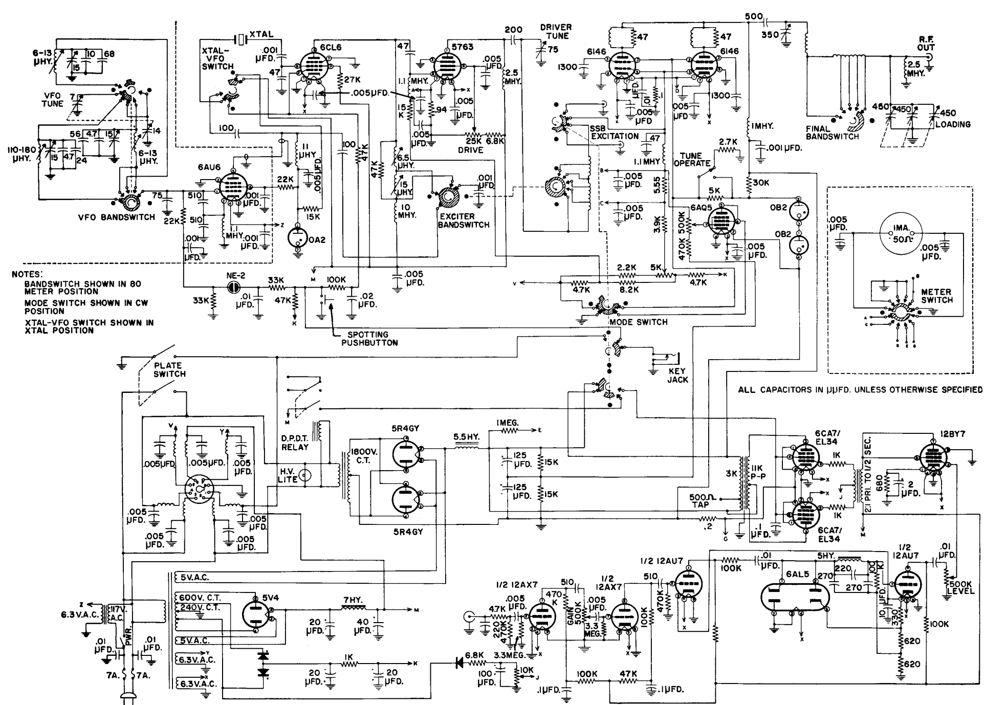
Heathkit "Apache" transmitter, from Radio & TV News, April 1959
