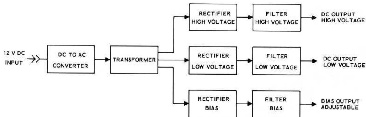
BLOCK DIAGRAM
