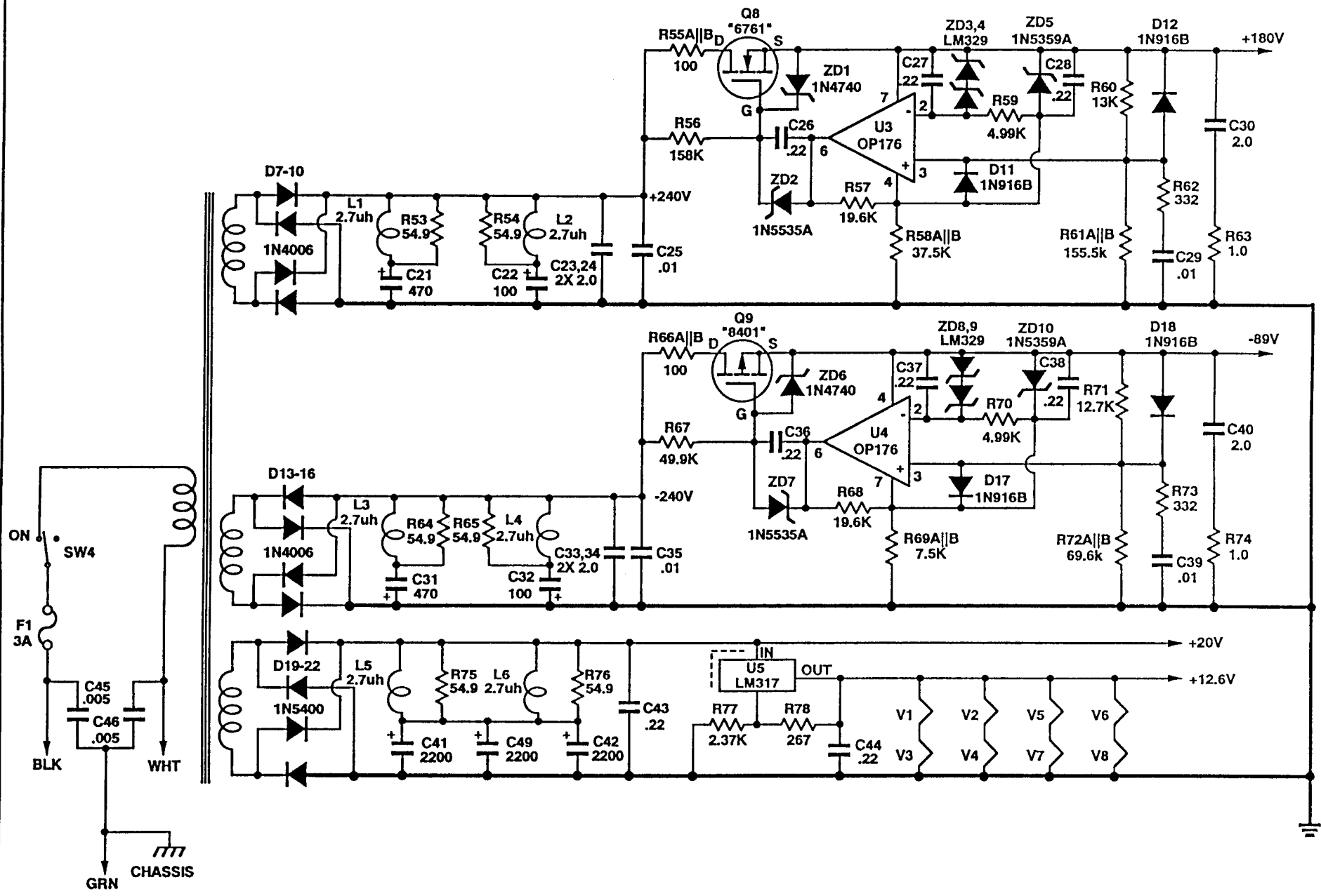
LS22 PREAMPLIFIER POWER SUPPLY PAGE 3 OF 3 6-23-95
