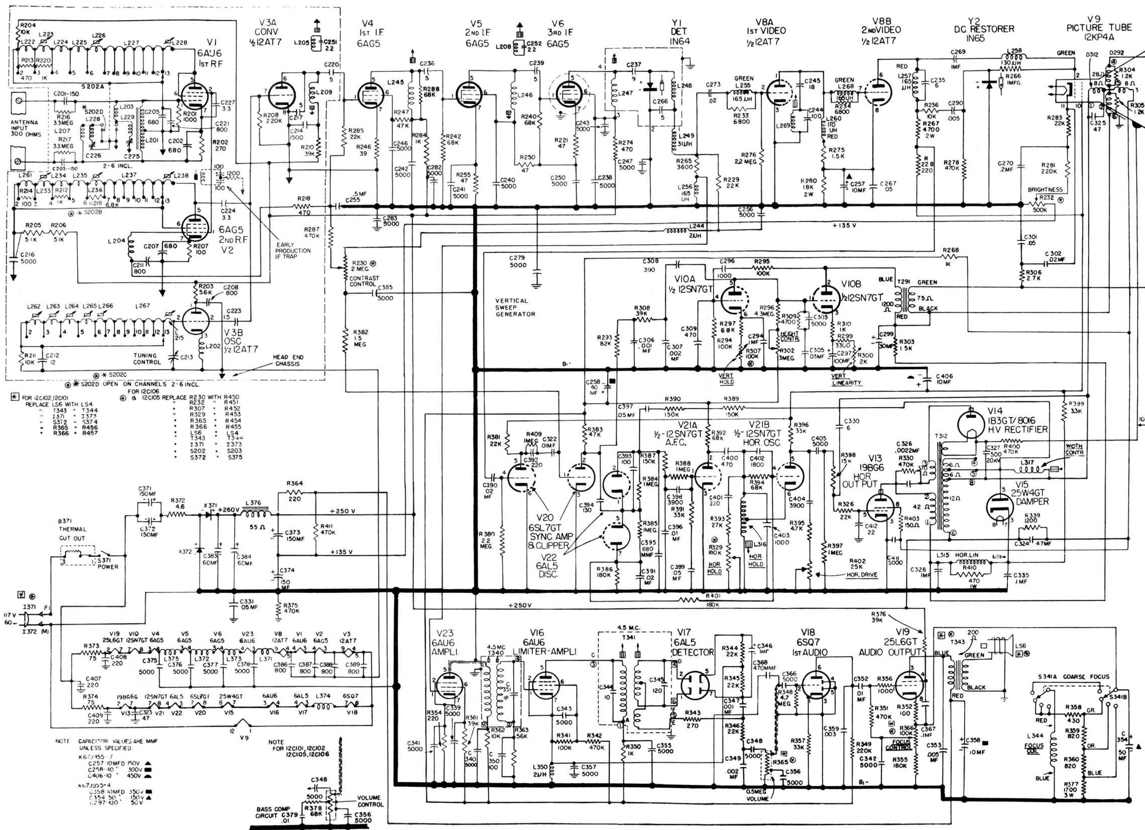
FIG. 9. SCHEMATIC DIAGRAM - MODELS 12T1, 12T2, 12C101, 12C102, 12C105
