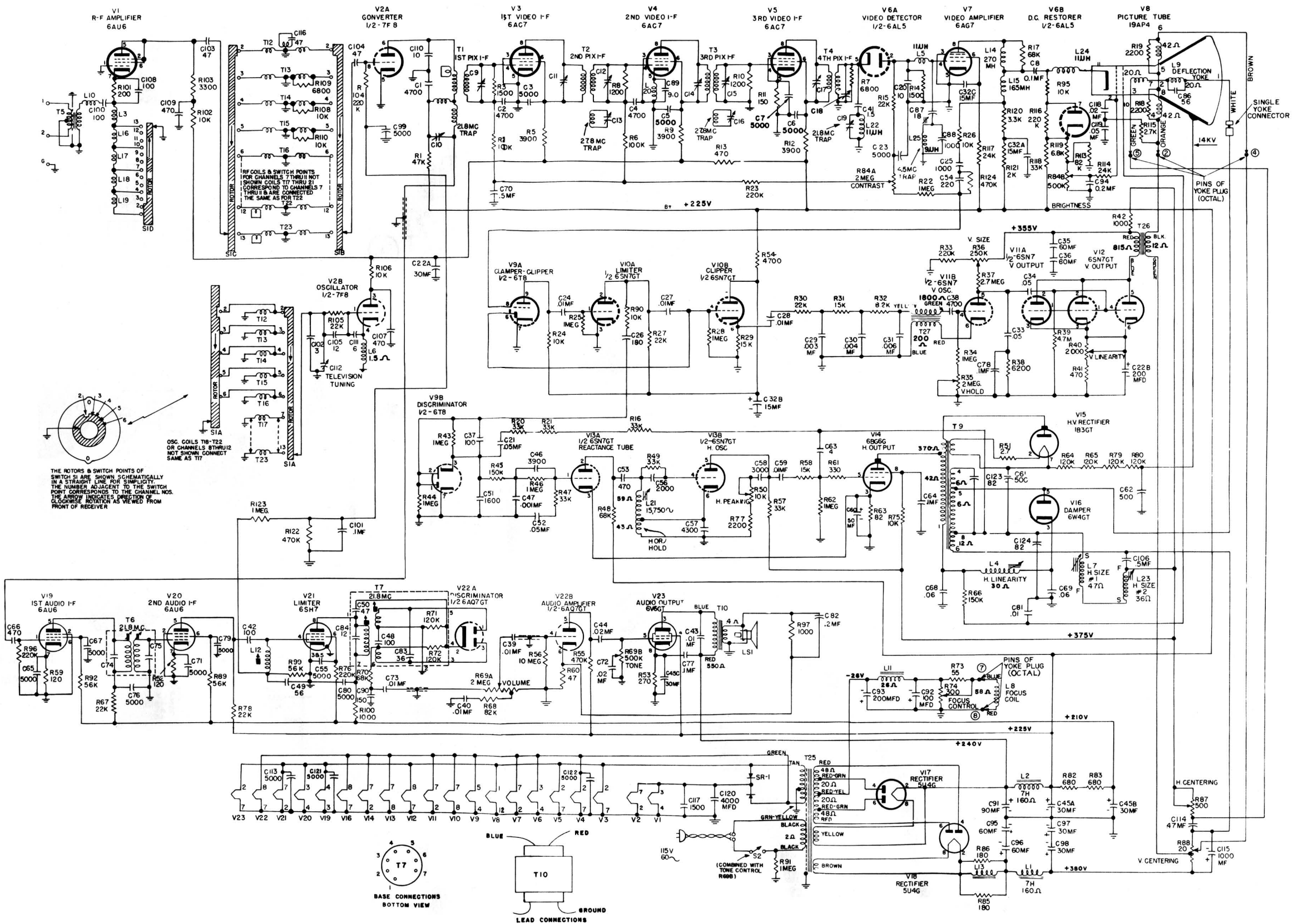
Fig. 13. Schematic Diagram, Model 19C10
