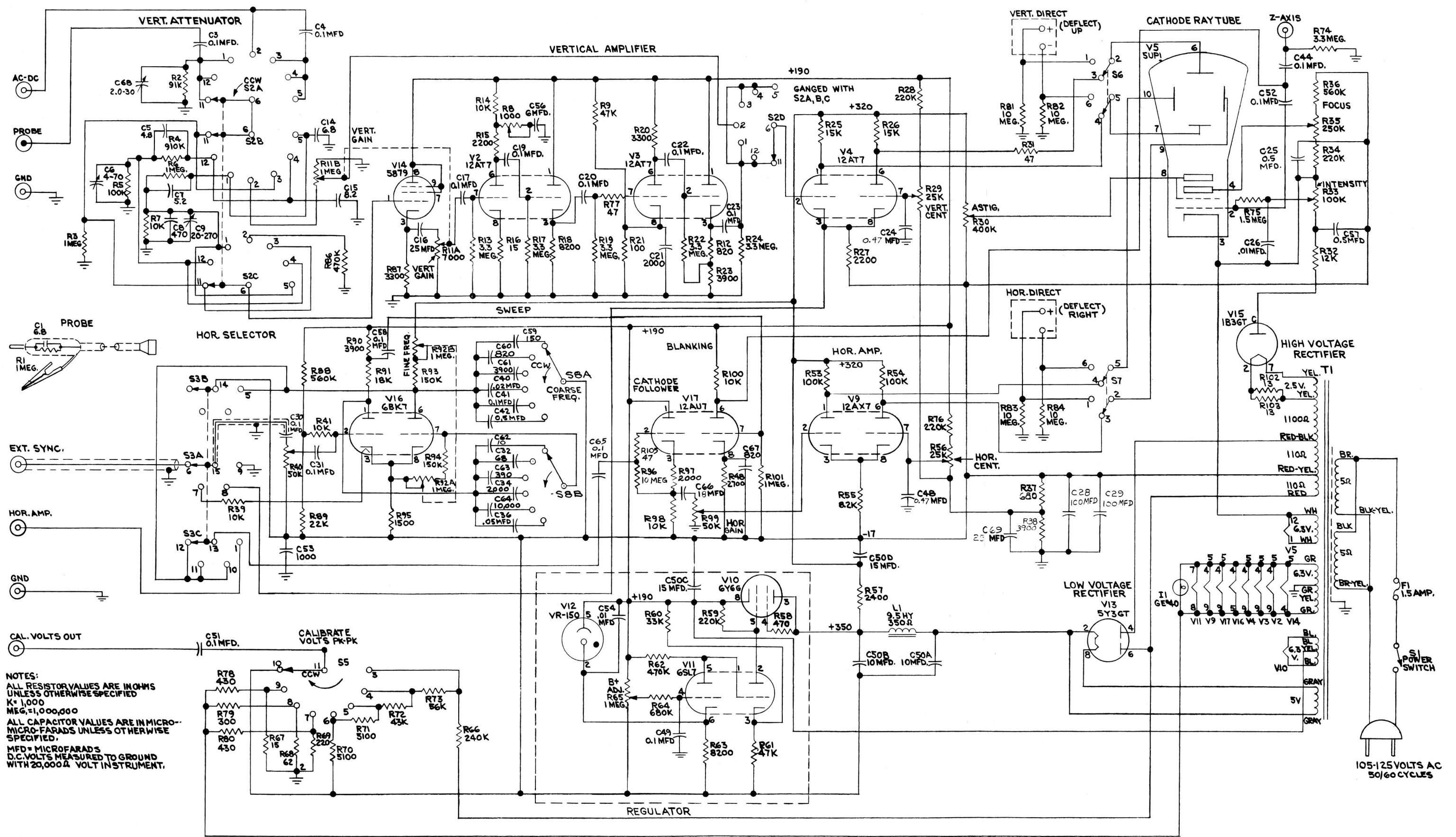
Fig. 24 Elementary Diagram, Oscilloscope, Model 4ST2A3, Revision B (E-7354104, Rev. 5)
