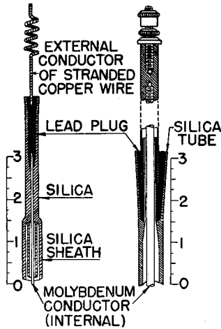
Fig. 2—Silica seals.
