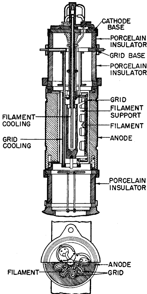
Fig. 13—Inner structure of the 500-kilowatt Metropolitan-Vickers tube.
